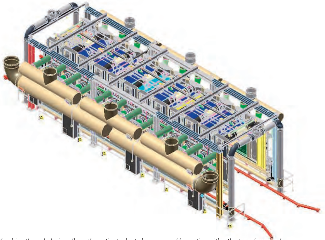
The drive-through design allows the entire trailer to be processed by section within the tunnel surround.
